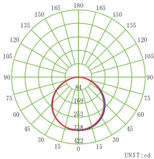
12W 6" Round LED Downlight LUMINOUS INTENSITY DISTRIBUTION DIAGRAM
