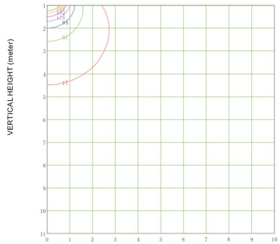
VERTICAL EQUILUMINUS CURVE
